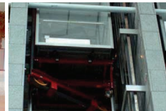
MP GLASS lift Grand Canal Dublin, Ireland Lifts: 4 MP2016G "S" Tailor-made cabins
